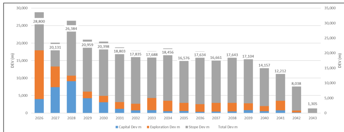
Figure 16.14: Development Schedule over LOM
