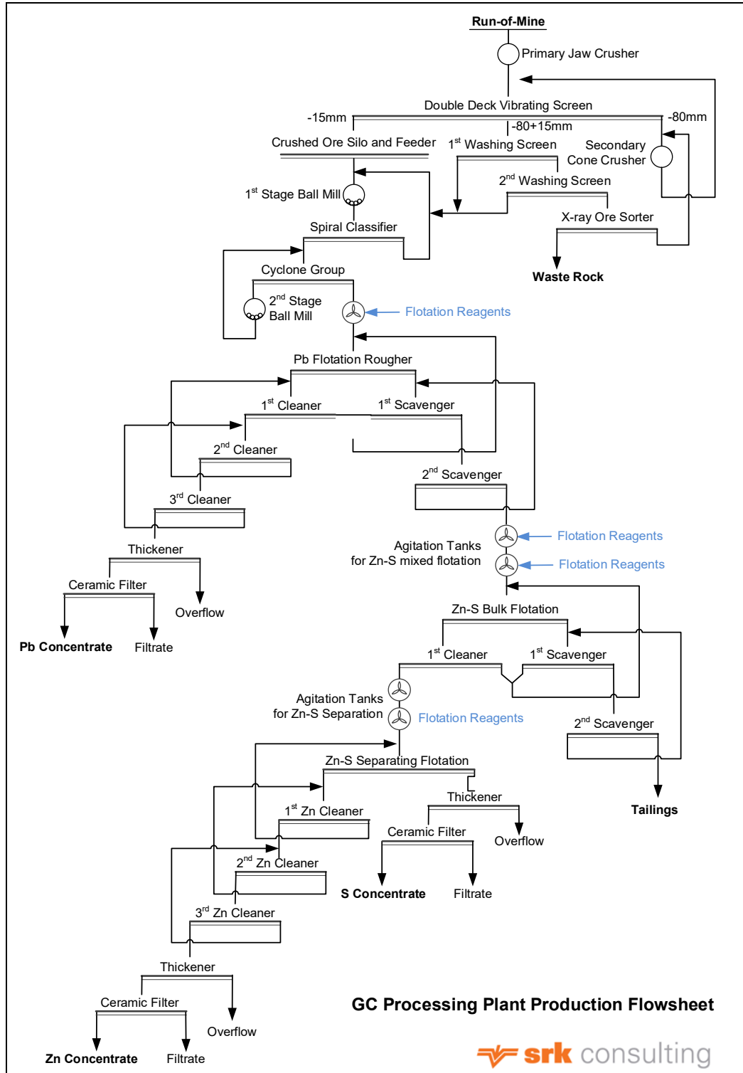
Figure 17.2: Production Process Flowsheet of GC Processing Plant
