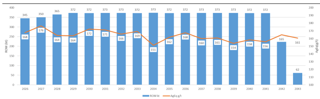
Figure 16.13: ROM Schedule over LOM
