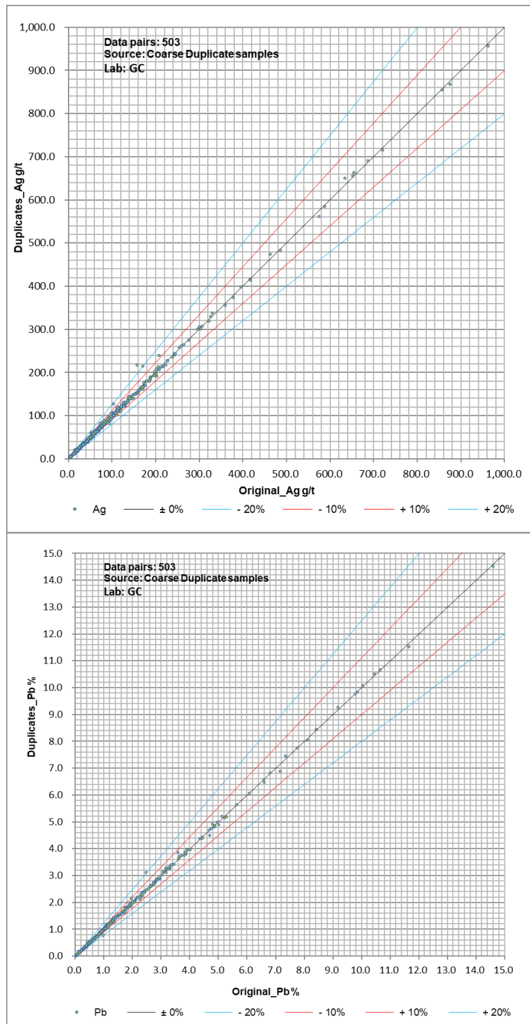
Figure 11.8: Scatter Plot of Coarse Duplicates
