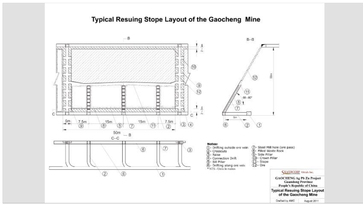
Figure 16.5: Typical Resuing Stope Layout
