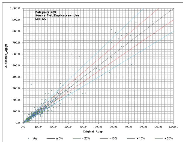
Figure 11.7: Scatter Plot of Field Duplicates
