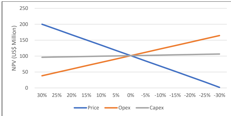
Figure 22.3: Sensitivity Spider Chart (8% Discount Rate)
