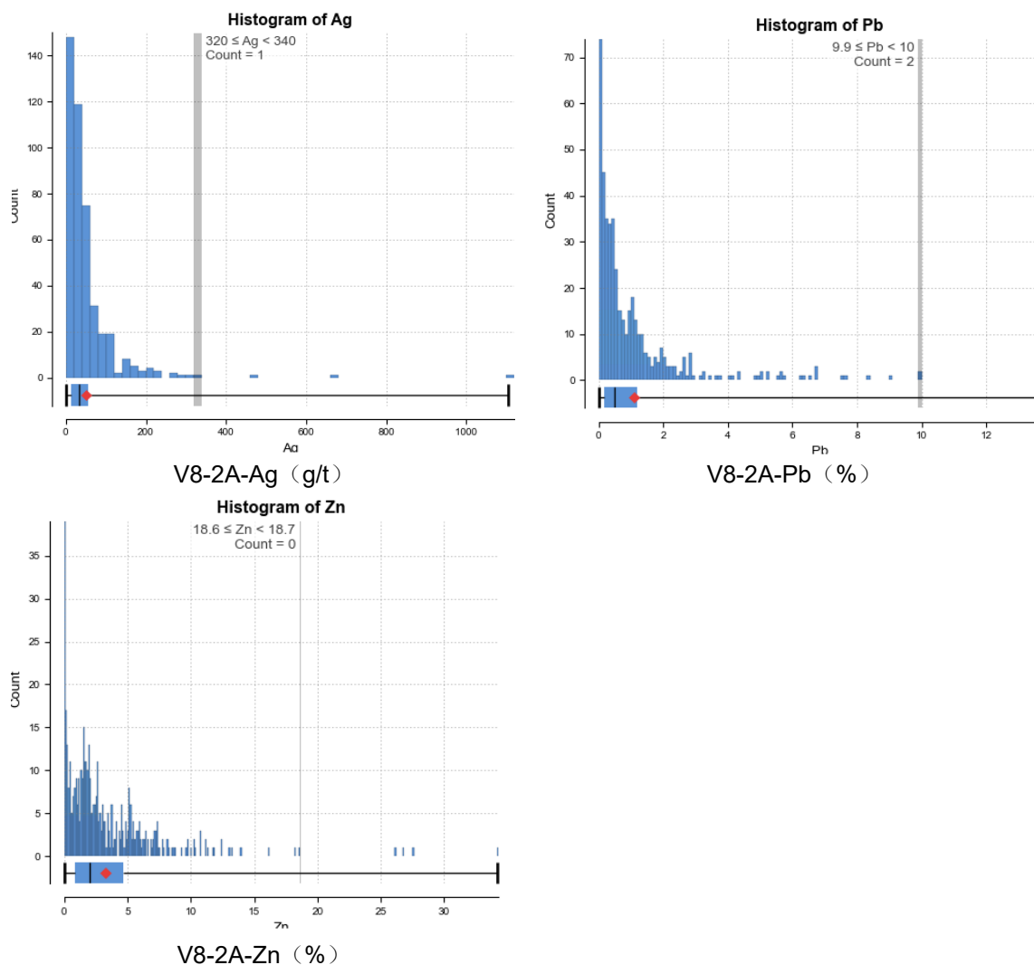
Figure 14.5: Histogram Plots for the Selected 10 Veins
