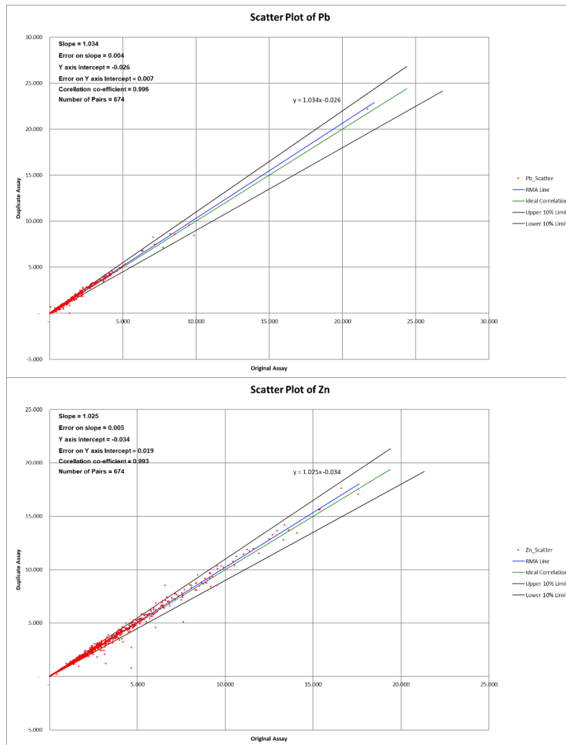
Figure 11.10: Scatter Plot of Umpire Samples from 2024 to 2025
