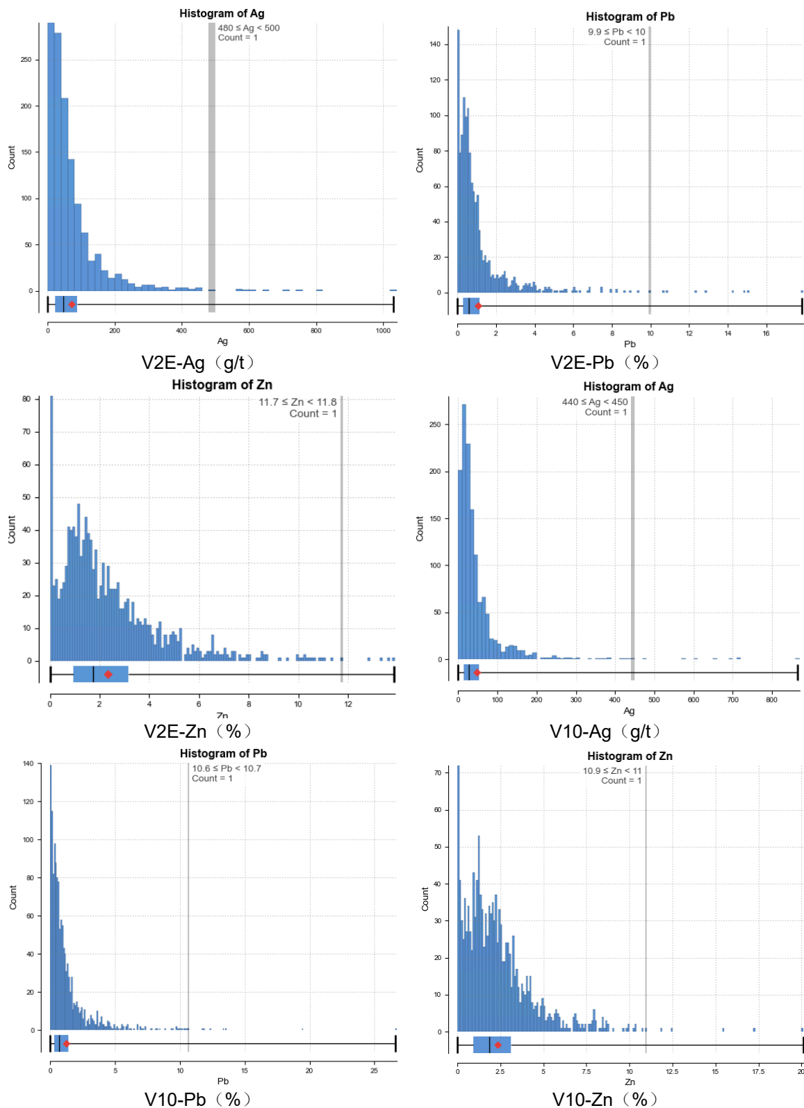
Figure 14.5: Histogram Plots for the Selected 10 Veins
