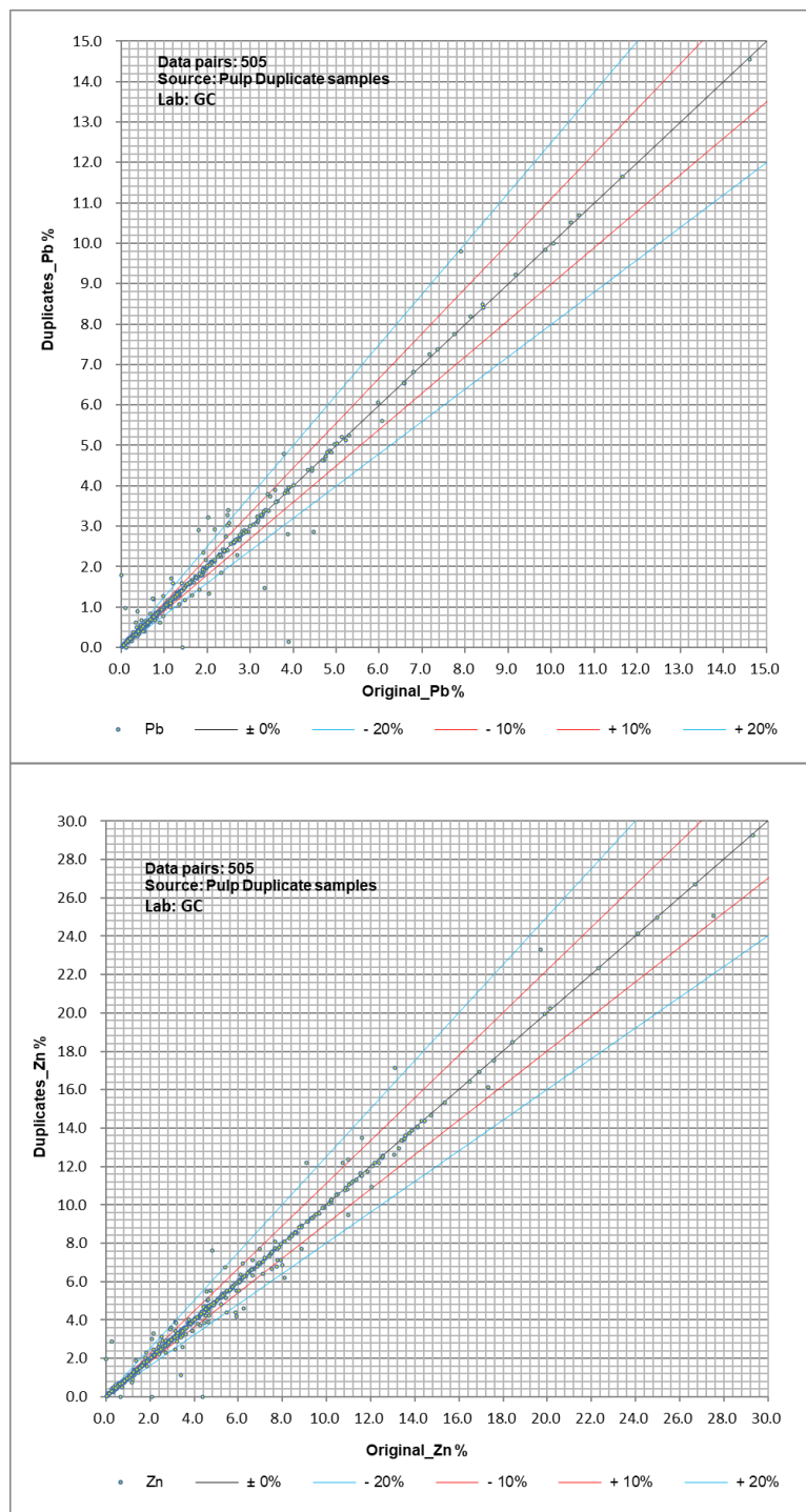
Figure 11.9: Scatter Plot of Pulp Duplicates
