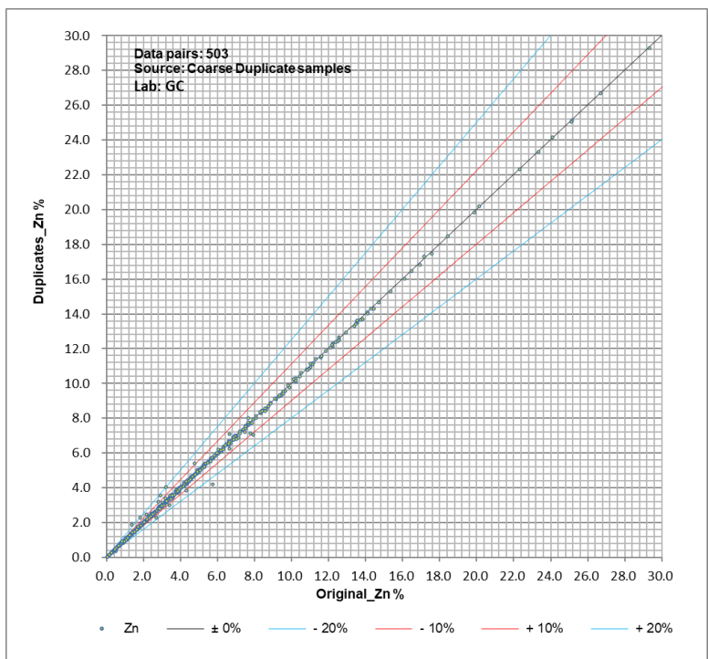
Figure 11.8: Scatter Plot of Coarse Duplicates
