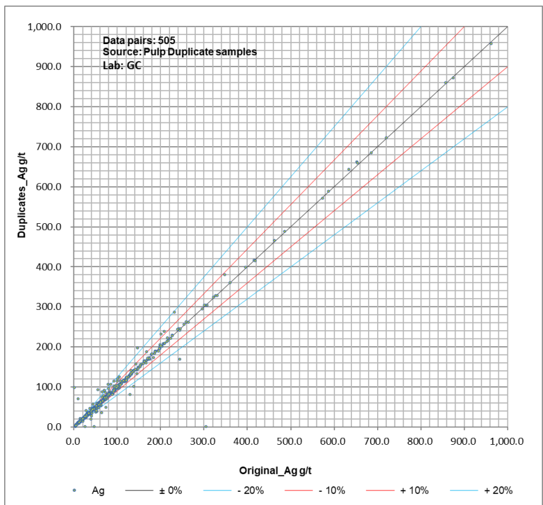
Figure 11.9: Scatter Plot of Pulp Duplicates
