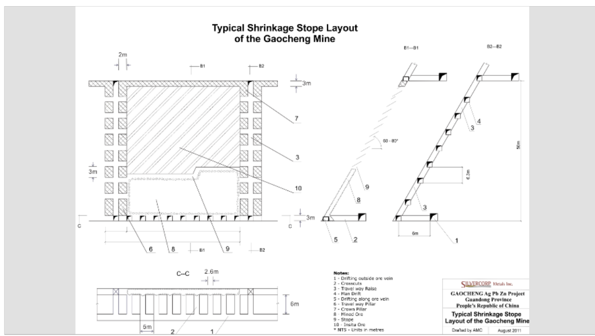
Figure 16.4: Typical Shrinkage Stope Layout
