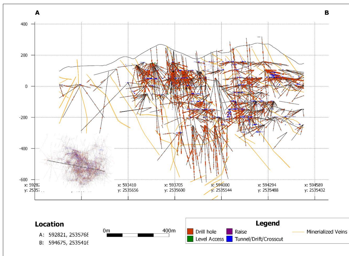
Figure 14.2: Mineralized Veins Section
