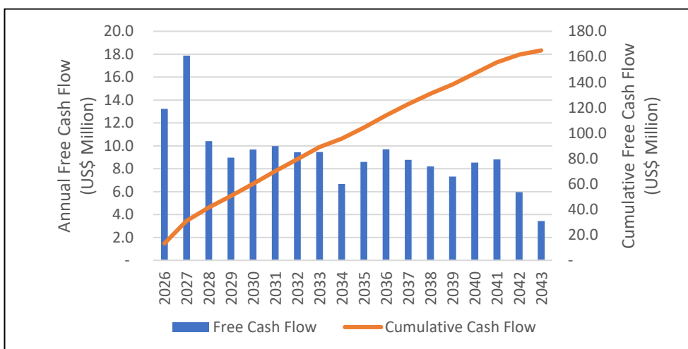
Figure 22.1: Cash Flow Profile
