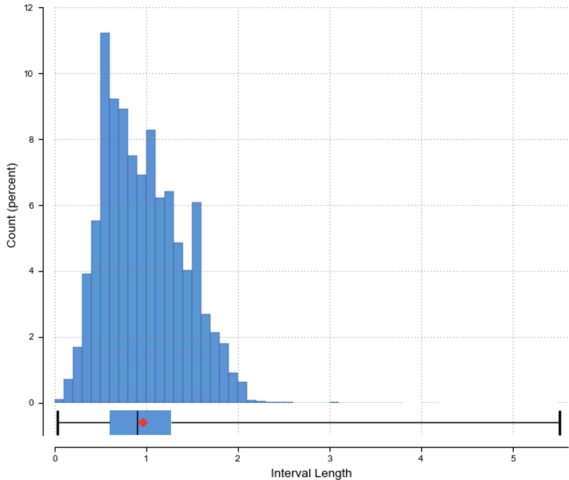
Figure 14.4: Sampling Interval Histogram
