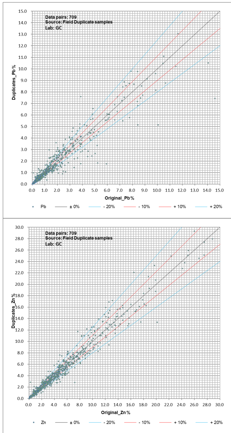
Figure 11.7: Scatter Plot of Field Duplicates
