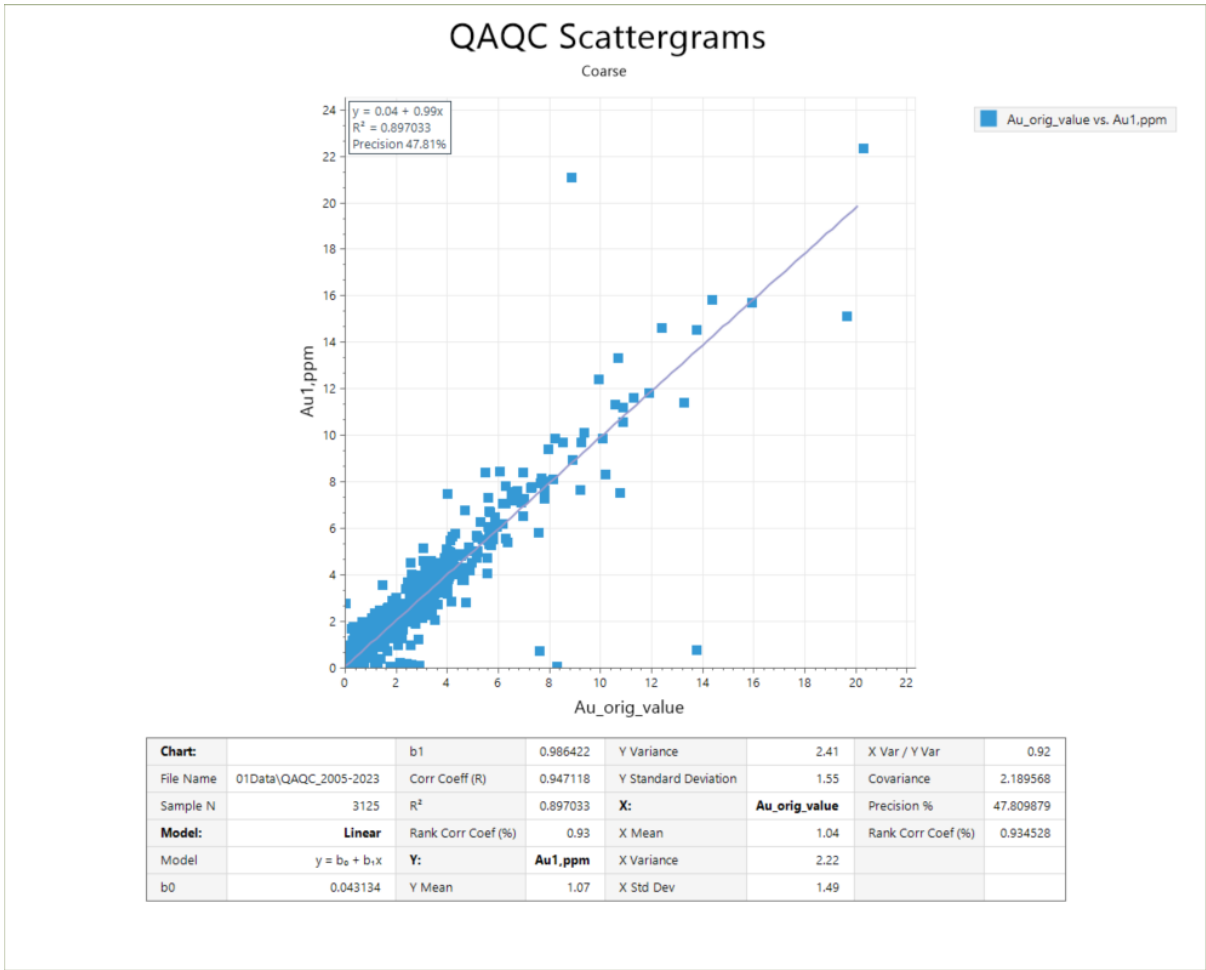
Figure 11.9: QAQC Program, Coarse Duplicate Results.
