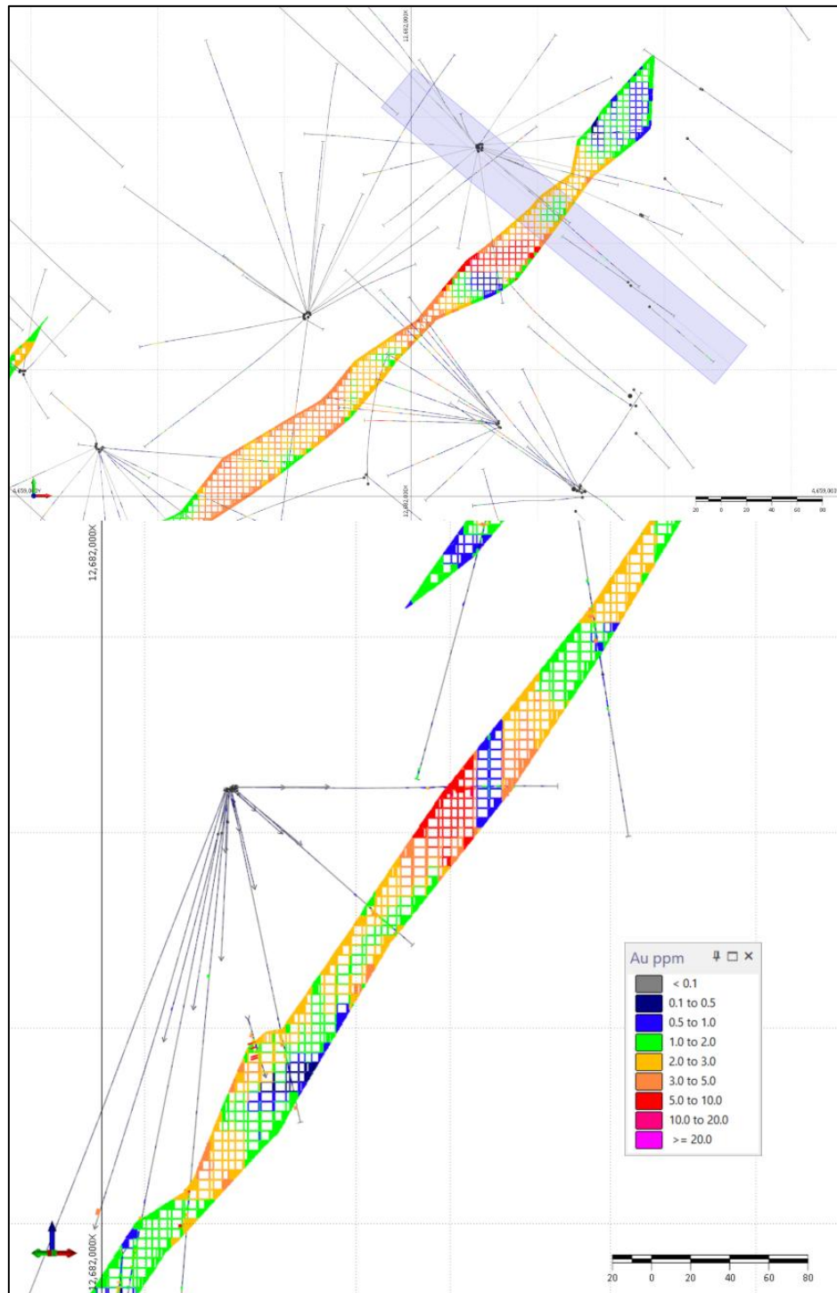
Figure 14.19: Kyzyltash, Au, contact zone (clipping \pm 20\text{m} ) section NE-SW.
