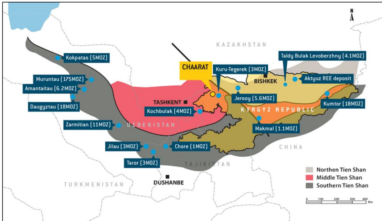
Figure 7.1: Chaarat Project Location in Tien Shan Belt.
