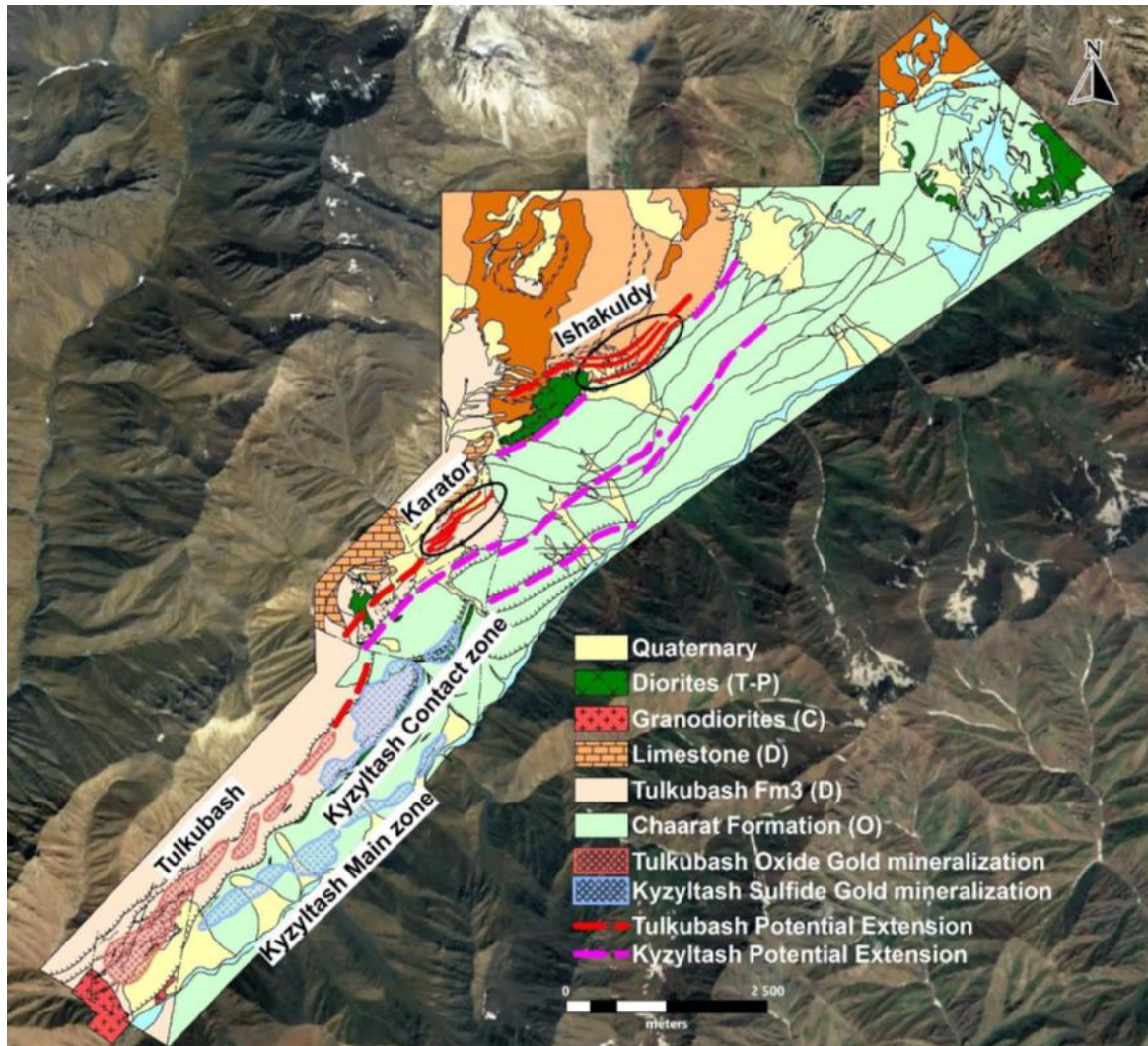
Figure 7.3: Chaarat ore field, Sandalash Shear zone, geology and mineralization.
