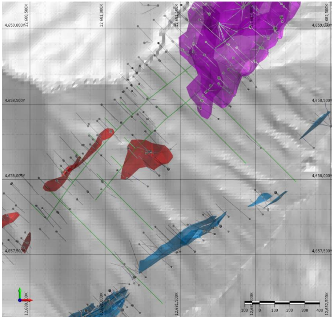
Figure 26.1 Plan view of planned underground Tunnel for Contact Zone Extension
