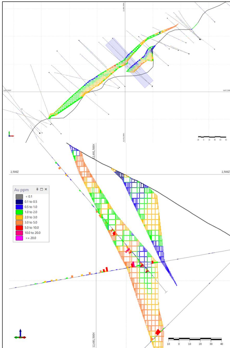
Figure 14.18: Kyzyltash, Au, Main Zone (clipping \pm 20\text{m} ) level plan 2470ml.
