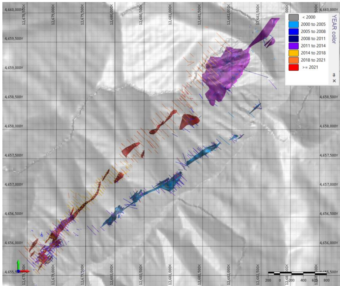
Figure 10.1: Plan map showing location of drill holes by year for Tulkubash and Kyzyltash deposits.
