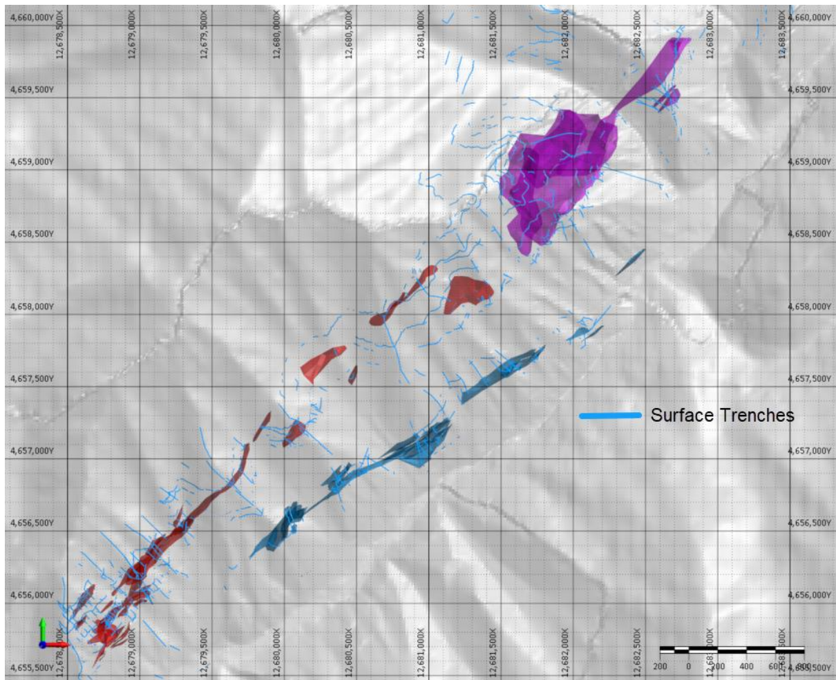
Figure 9.2: Surface trenching across the Chaarat Gold project area.
