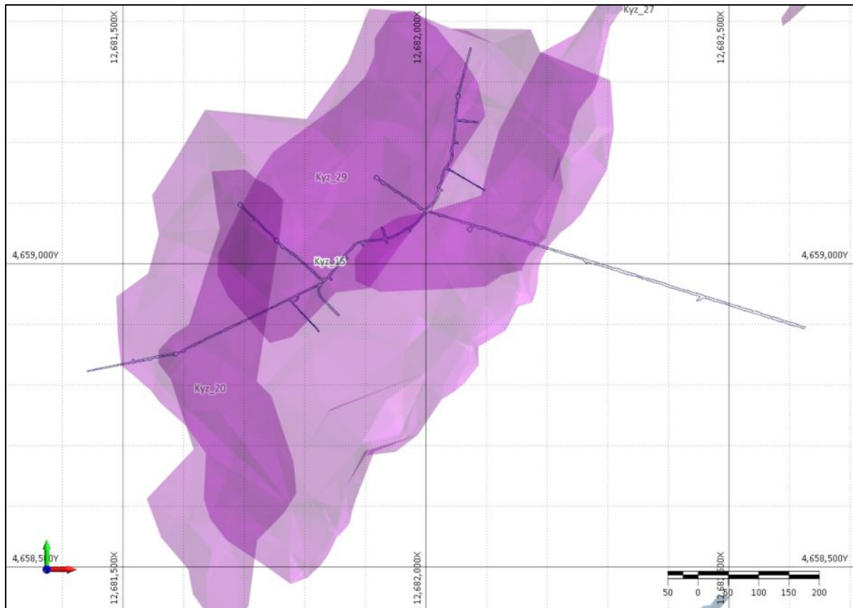
Figure 9.3: Kyzyltash Contact Zone adit 4, total length approximately 2.1km
