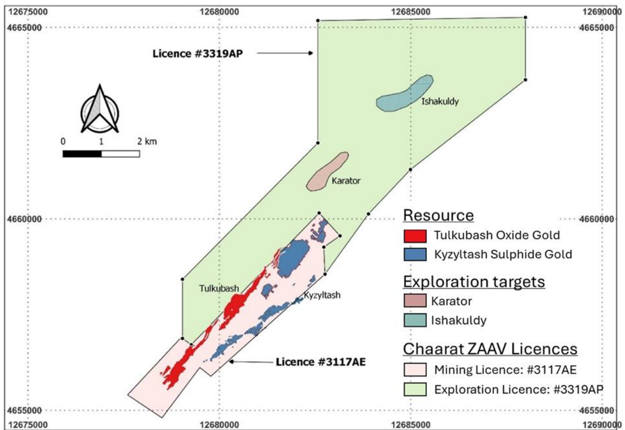
Figure 4.3: License map of Chaarat Gold Project.
