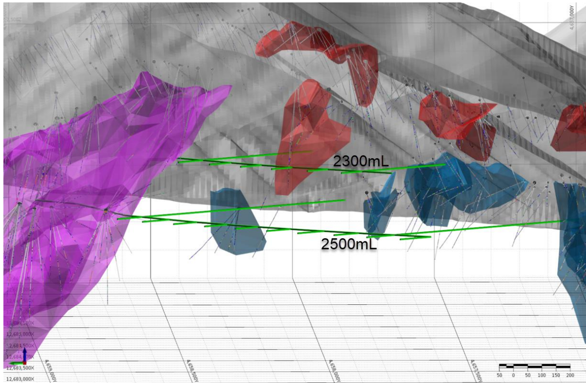
Figure 26.2 Rotated view of planned underground Tunnel for Contact Zone Extension
