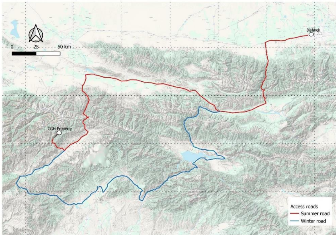
Figure 5.1: Location of the Chaarat Gold Project and access routes.
