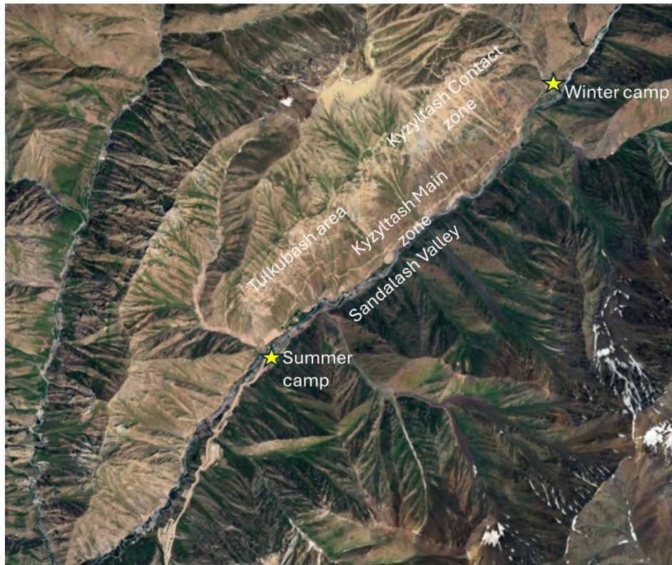
Figure 9.1: Chaarat Gold Project, Satellite image, Google Earth 02/2026.
