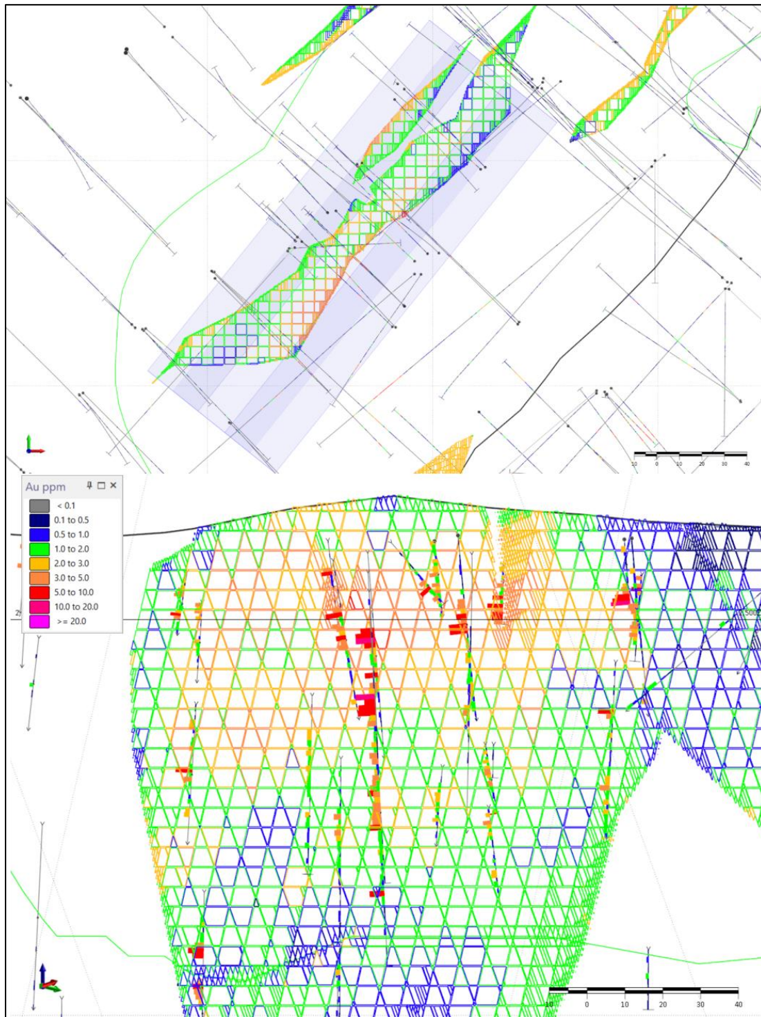
Figure 14.17: Tulkubash, Au, Main Pit Area (clipping \pm 15\text{m} ) long section.
