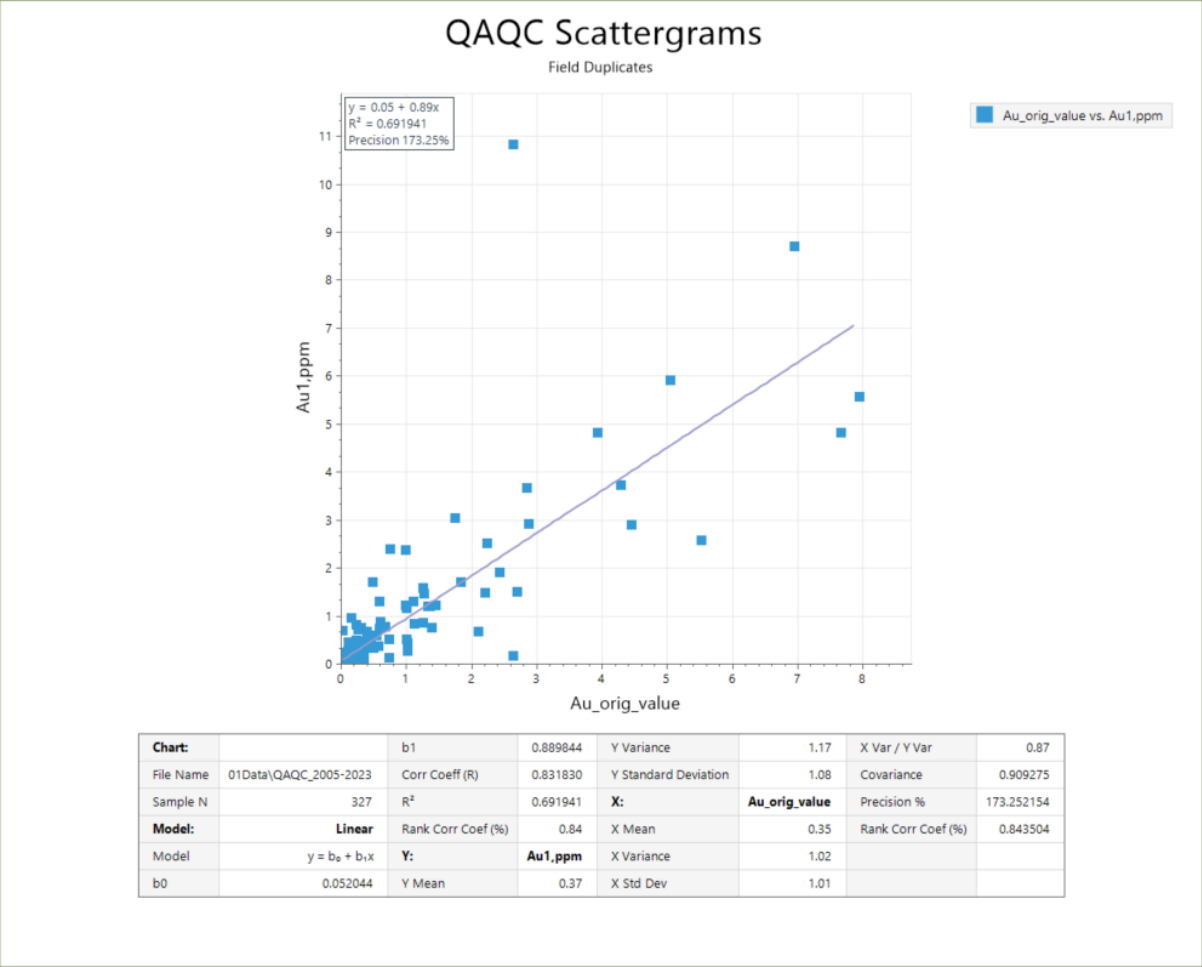
Figure 11.11: QAQC Program, Field Duplicate Results.
