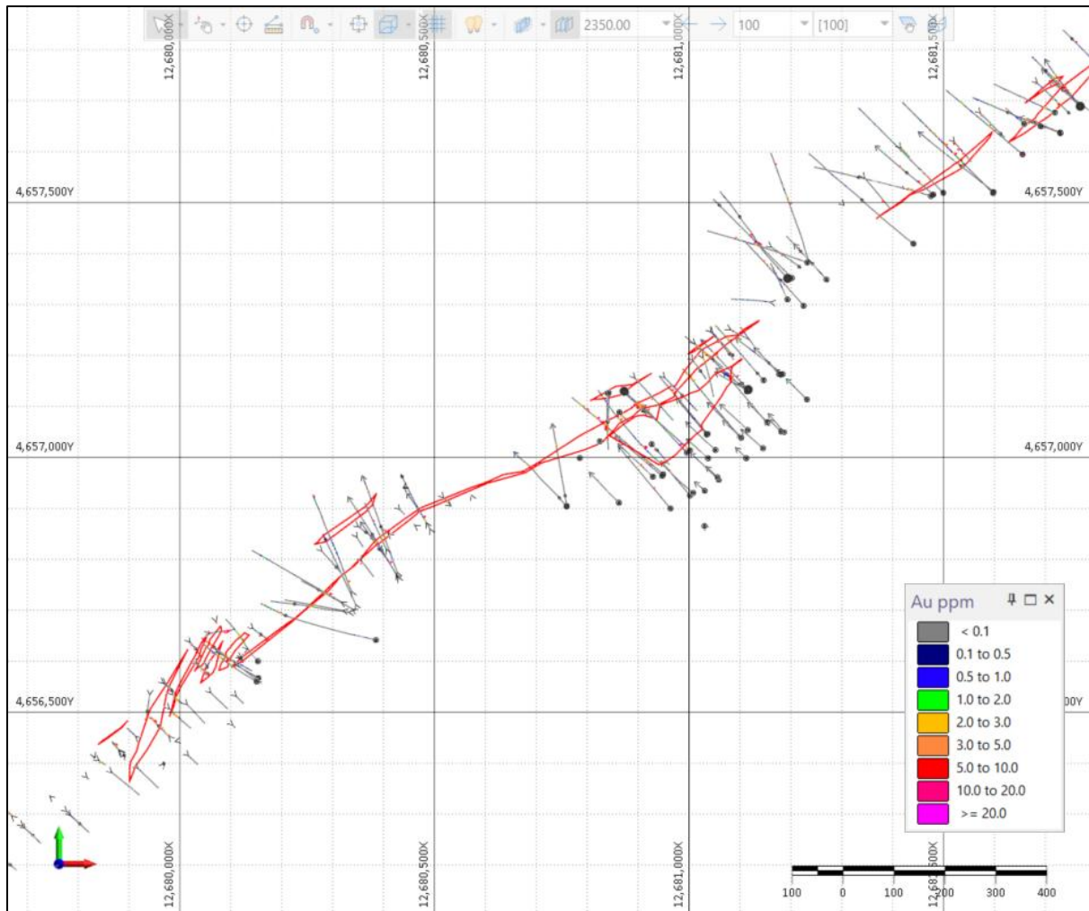
Figure 14.4: Planview of Kyzyltash Main Zone, drill holes used in the current resource estimation, ore sliced at 2350ml with +/-100m clipping window.
