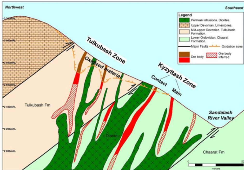
Figure 7.5: Chaarat project mineralization styles, Conceptual cross section.
