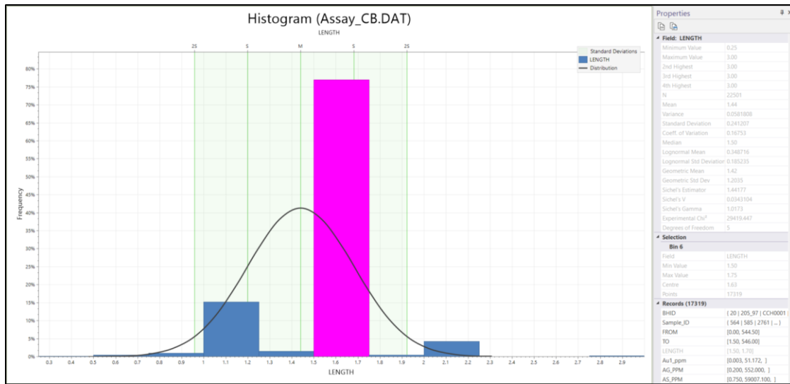
Figure 14.11: Histogram showing majority of samples of 1.5 m length.
