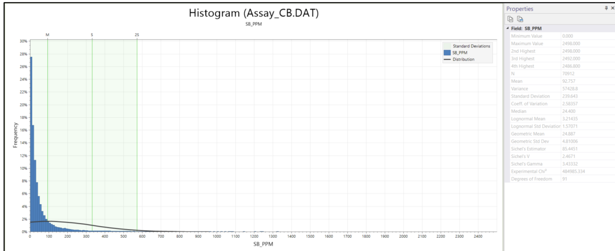
Figure 14.10: Histogram and frequency plot basic statistics (Sb ppm).
