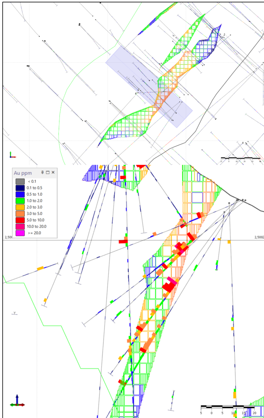
Figure 14.16: Tulkubash, Au, Main Pit Area (clipping \pm 20\text{m} ) Level Plan 2500ml Elevation.
