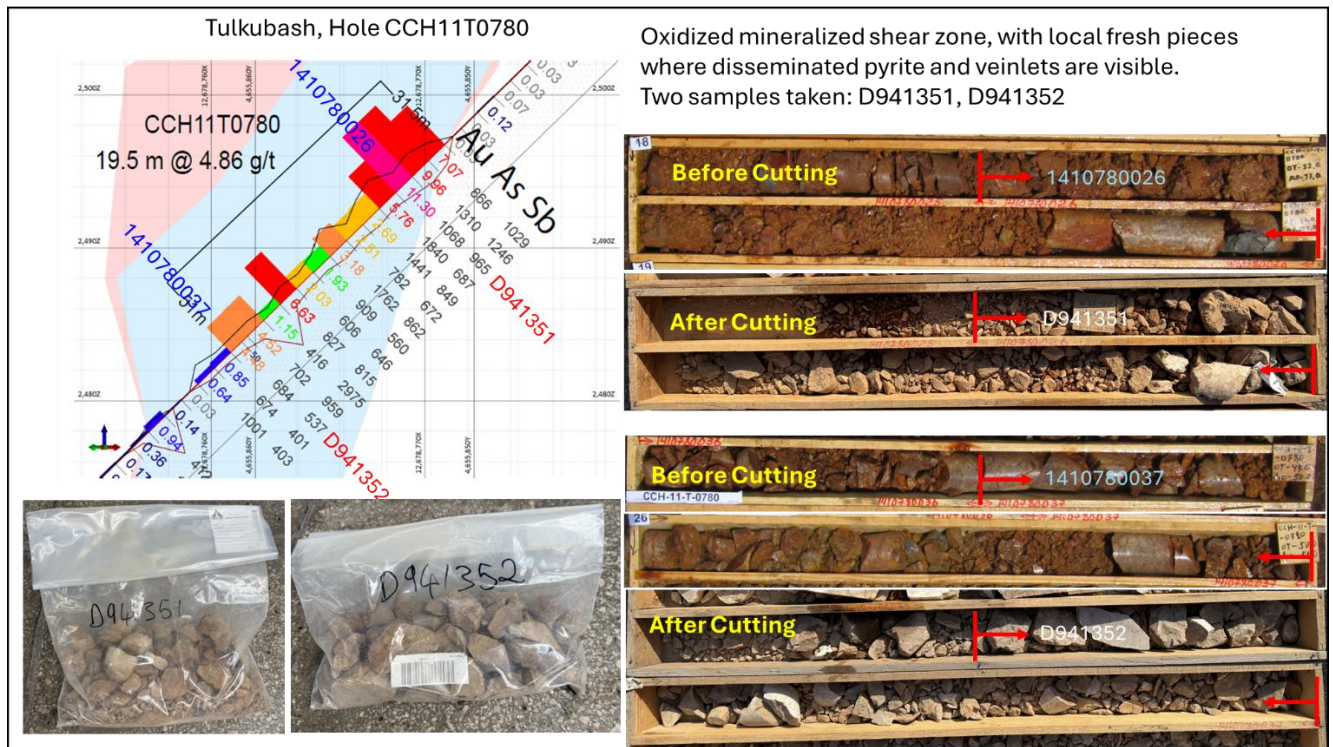
Figure 12.3: Close up of the interval selected for review, along with before and after images of the sample which were taken from the core boxes.
