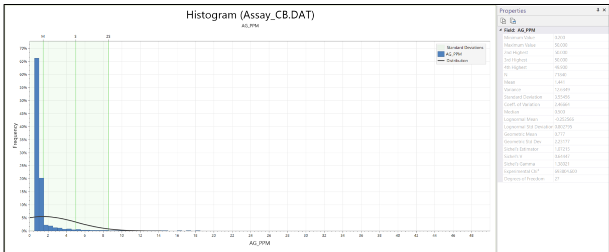
Figure 14.8: Histogram and frequency plot basic statistics (Ag ppm).
