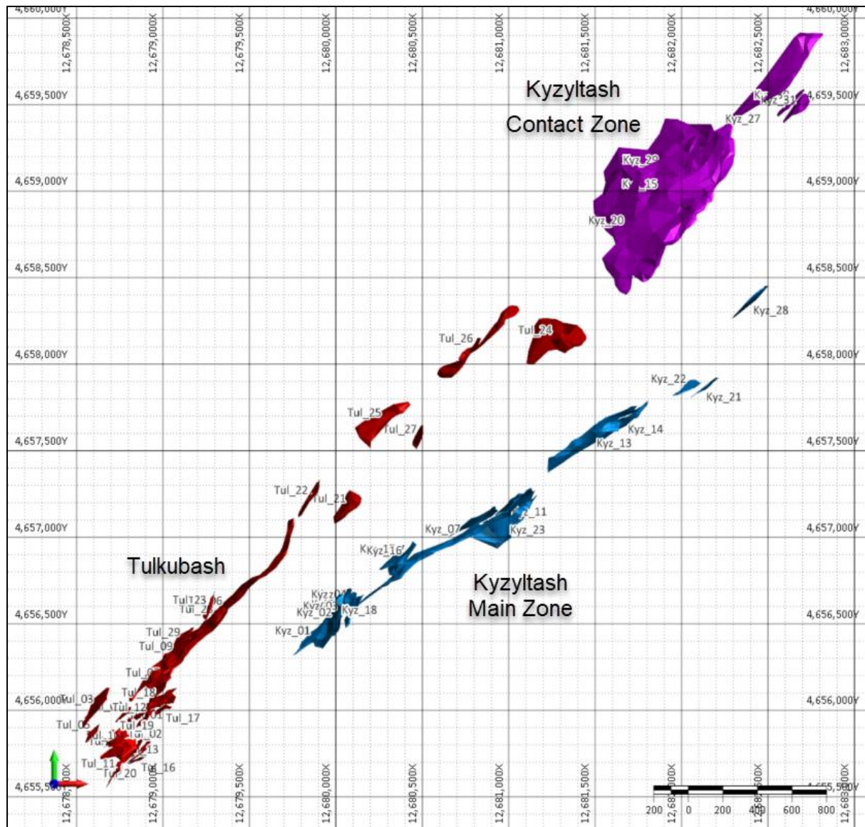
Figure 14.2: Spatial distribution of mineralized wireframes for Tulkubash and Kyzyltash deposits.
