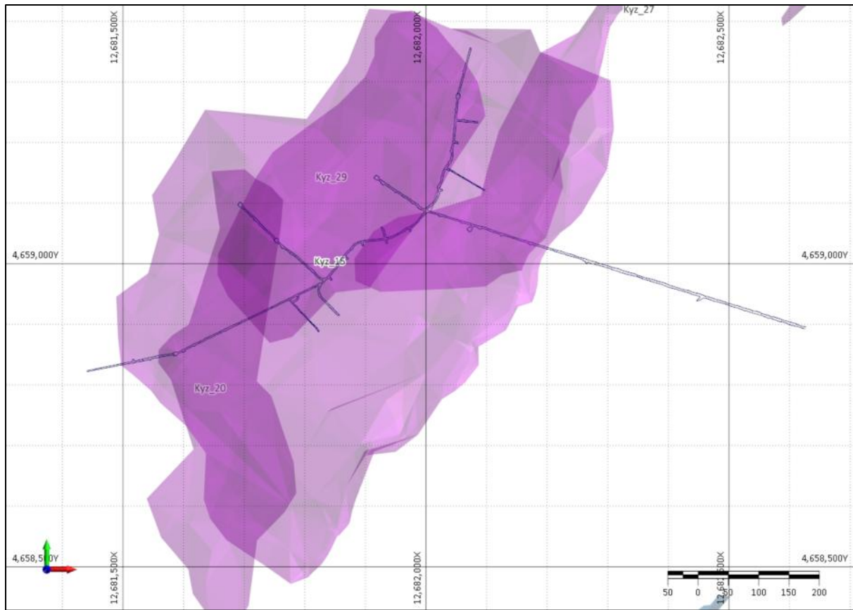
Figure 14.6: Contact Zone adit 4, total length of approximately 2.1 km
