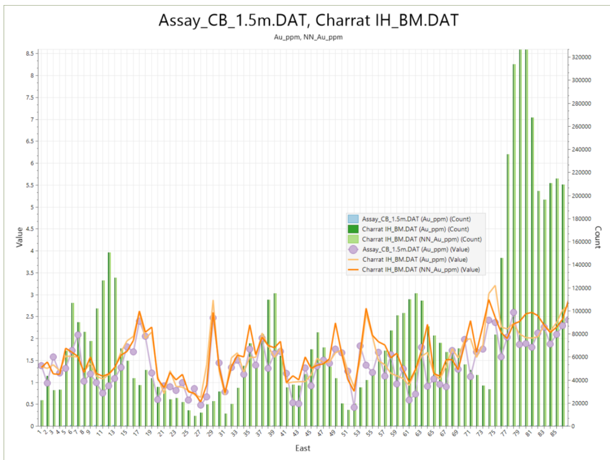
Figure 14.20: Swath plot, assay composites.
