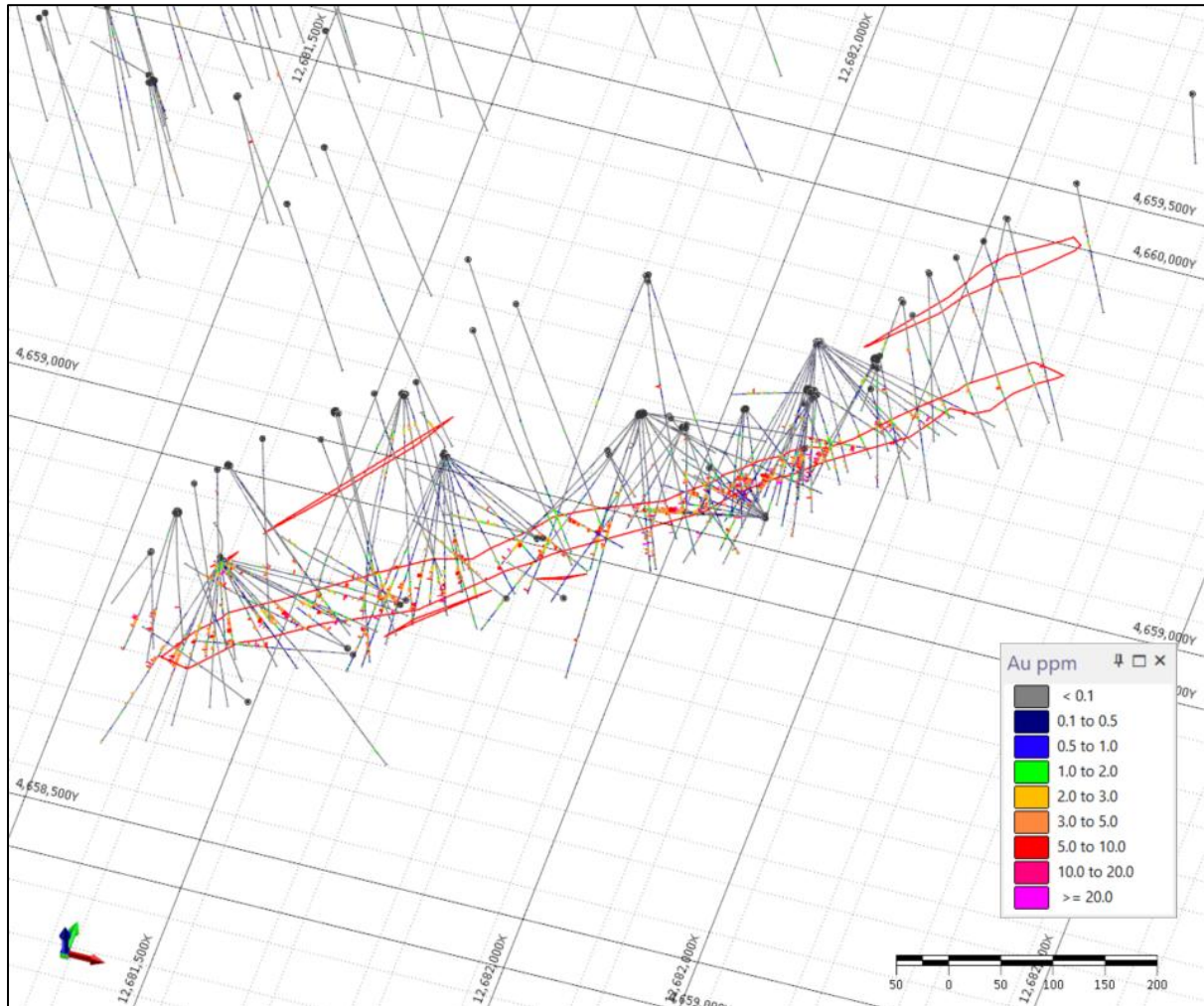
Figure 14.5: Kyzyltash Contact Zone, drill holes used in the current resource estimation, looking down dip through Kyz_15.
