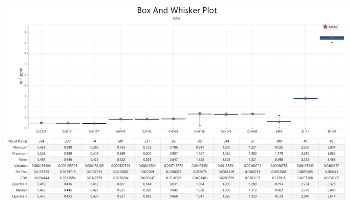
Figure 11.8: Box and whisker plot with base statistics for the CRM's results.
