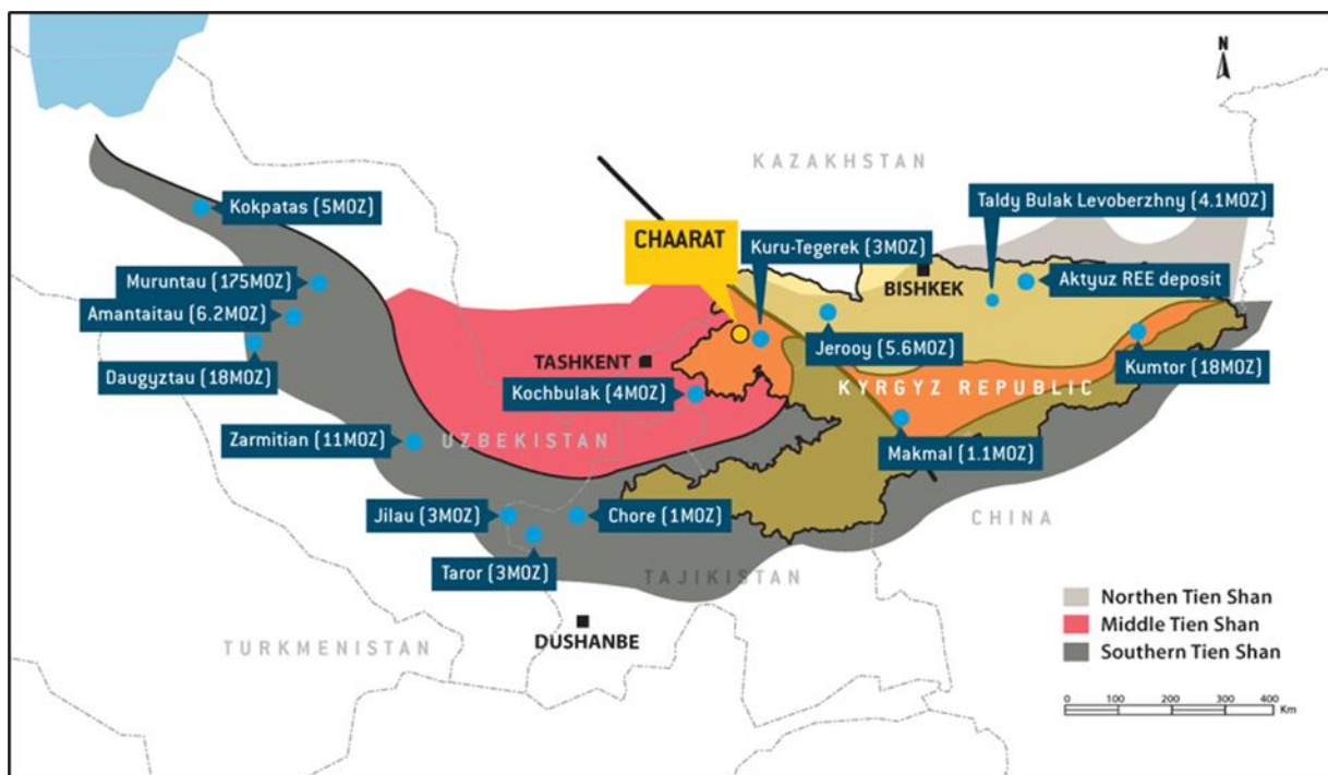
Figures 23.1: Chaarat Project Location in Tien Shan Belt and Mine map
