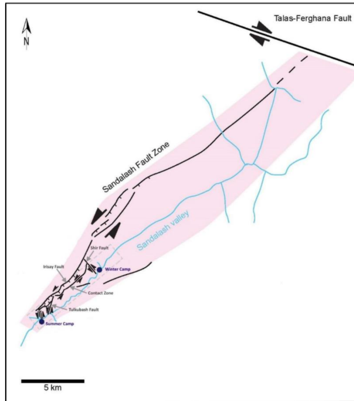
Figure 7.2: Chaarat ore field structural control, Sandalash Shear zone
