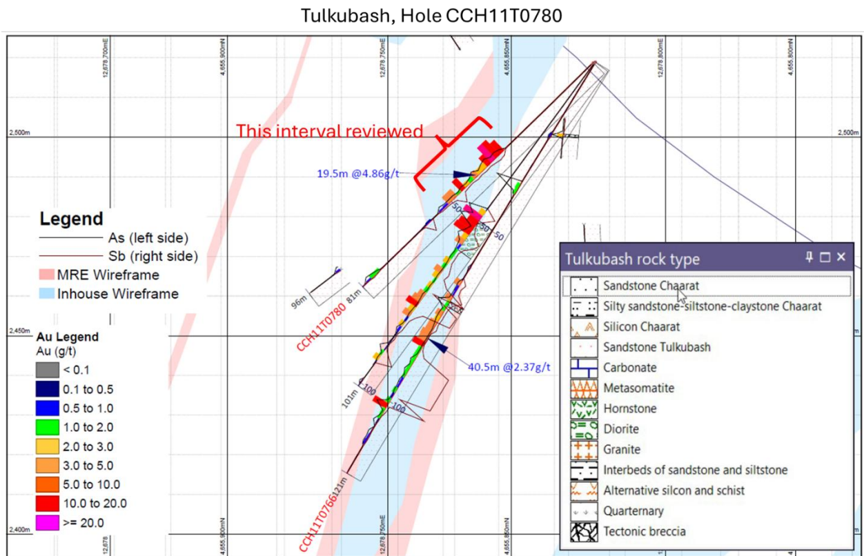
Figure 12.2: Representation of a mineralized interval selected for detailed review, verification, and check sampling from the Tulkubash deposit.
