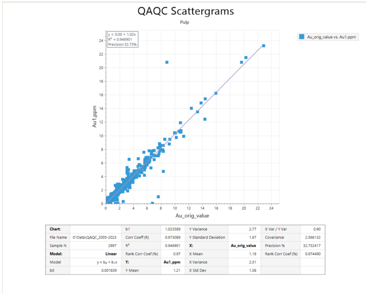
Figure 11.10: QAQC Program, Pulp Duplicate Results.
