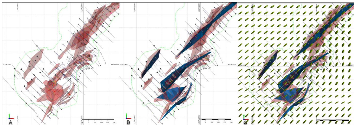
Figure 14.14: Tulkubash mineralization trend. A) Tulkubash Main pit area with 3D ore wireframes and drillholes, B) Trend surfaces created explicitly following main trends, C) Structural trend file created based on these trend surfaces with 50m grid cell size.
