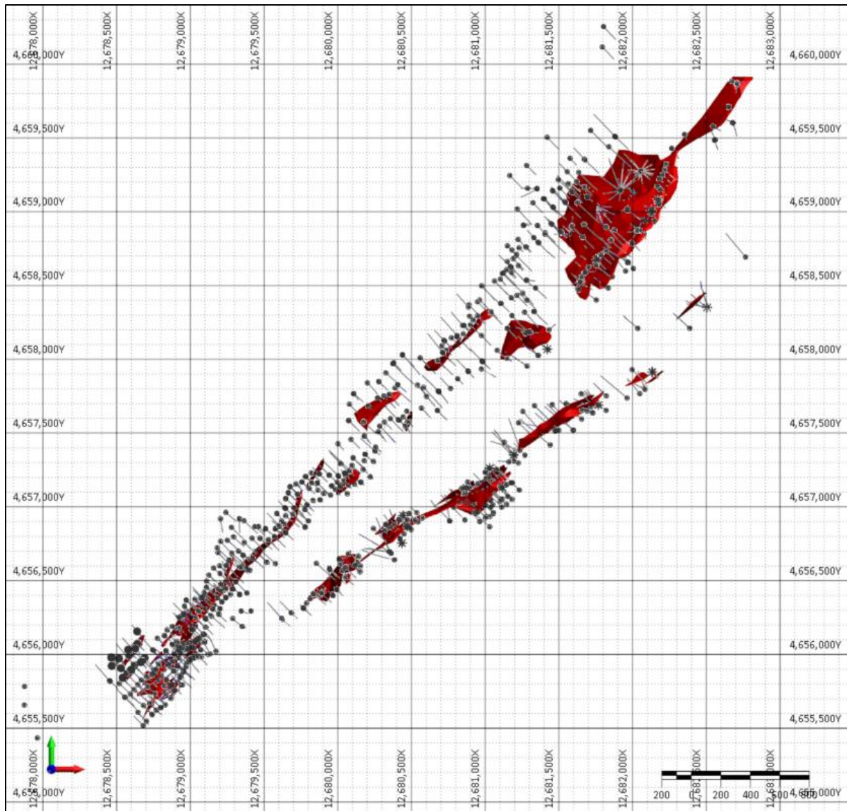
Figure 14.1: Planview of ore model 3D, and drill holes used in the current resource estimation.
