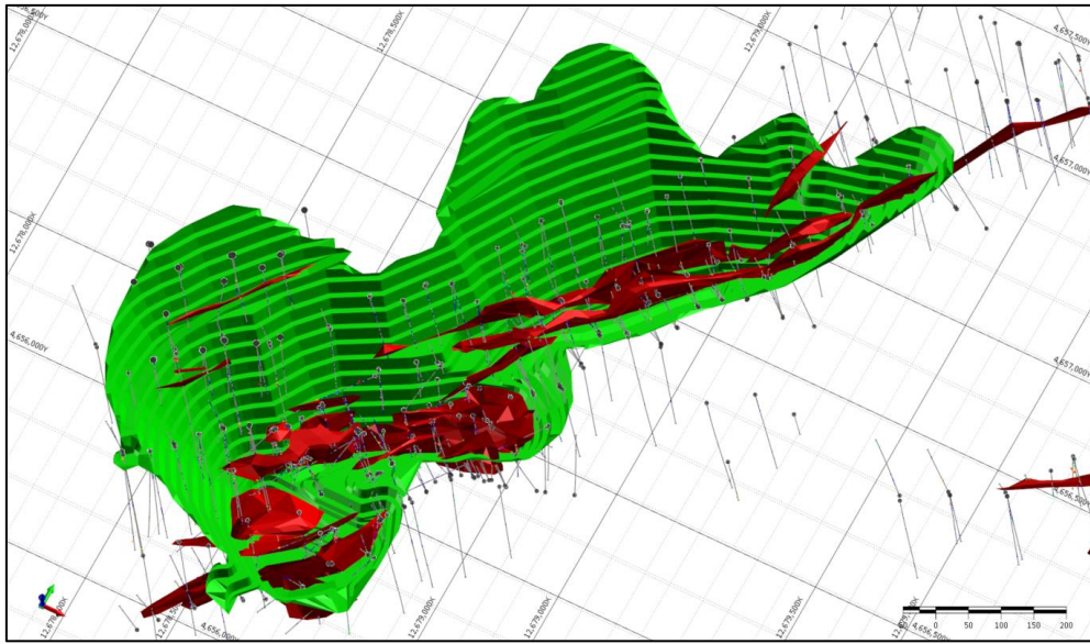
Figure 14.21: Tulkubash Pit shells.
