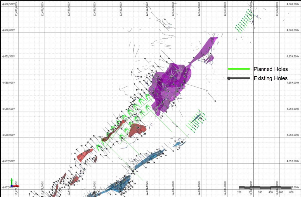
Figure 26.3 SVM planned drillholes.
