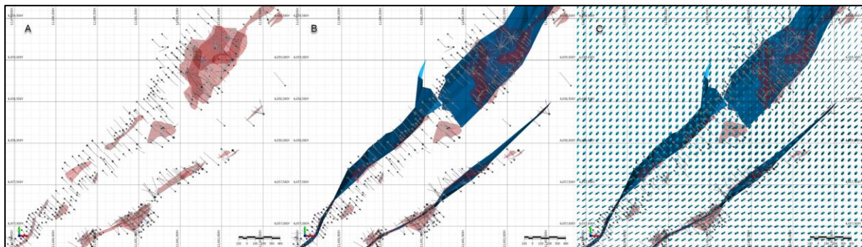
Figure 14.15: Kyzyltash mineralization trend. A) Kyzyltash main zone and contact zone with 3D ore wireframes and drillholes, B) Trend surfaces created explicitly following main trends, C) Structural trend file created based on these trend surfaces with 80m grid cell size.
