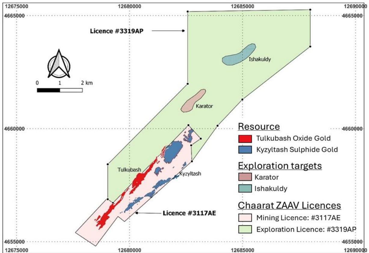
Figure 9.4: Location of the Karator and Ishakuldy exploration targets in relation to the main Tulkubash and Kyzyltash deposits.
