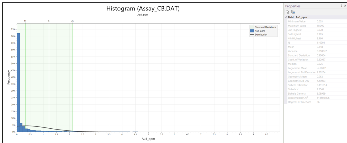
Figure 14.7: Histogram and frequency plot basic statistics (Au ppm).
