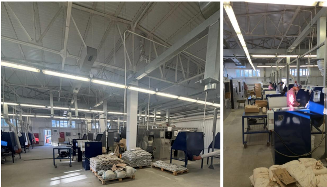
Figure 11.4: Sample crushing, splitting, and milling stations at Stewart Analytical and Environmental Laboratories.
