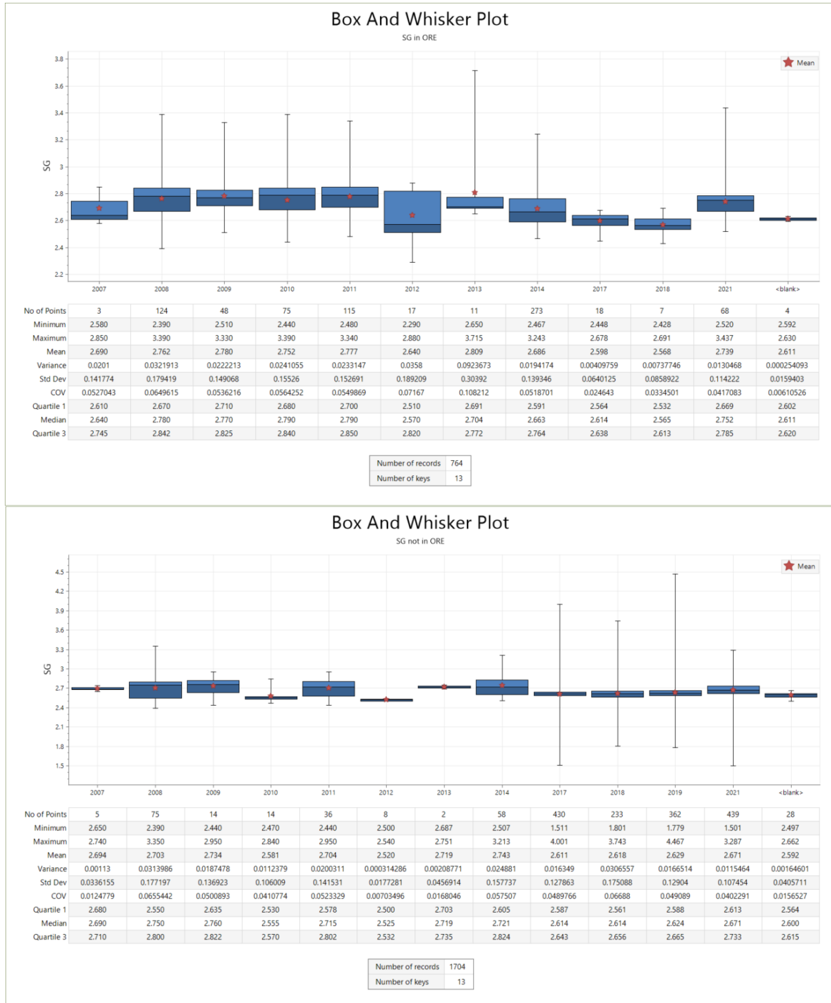
Figure 11.6: Density t/m 3
