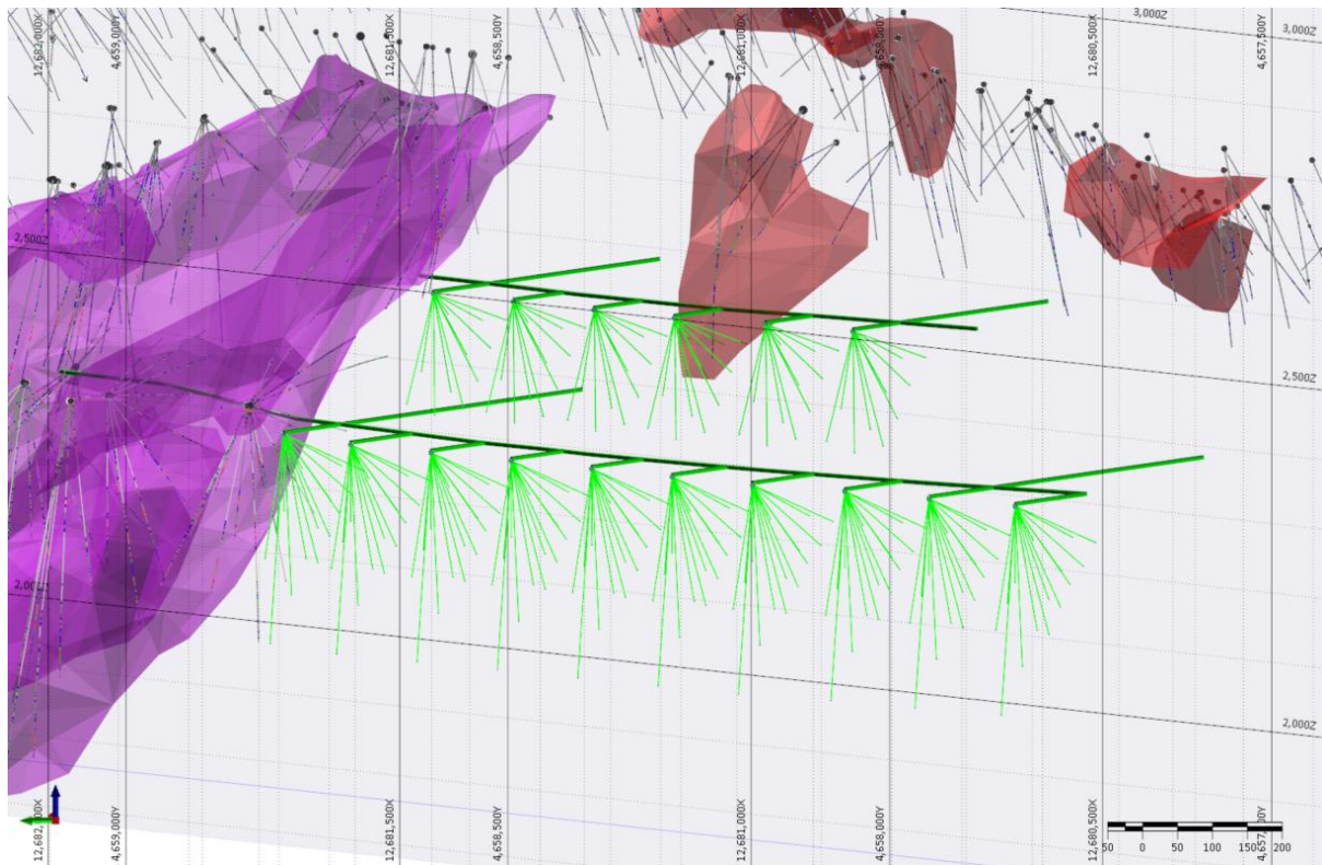
Figure 26.4 Planned drillholes from underground tunnels, Contact Zone extension.
