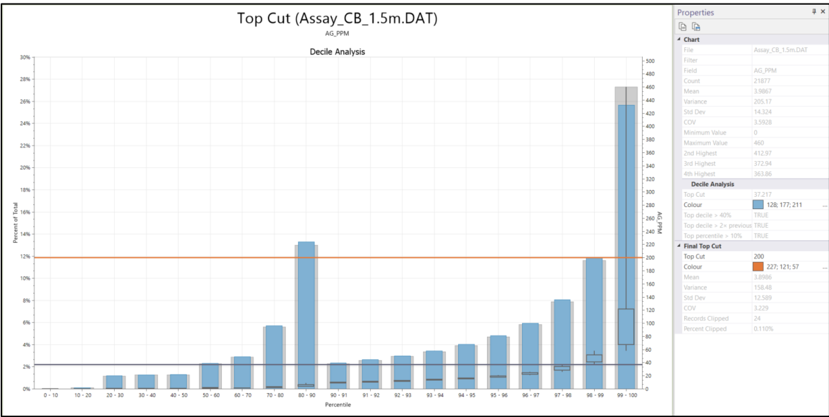
Figure 14.13: Decile analysis showing the top cut statistics for Ag.
