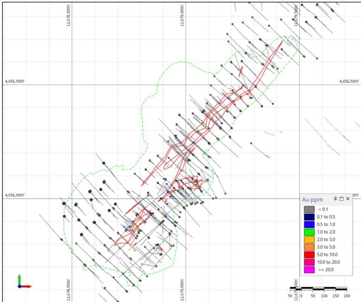
Figure 14.3: Planview of Tulkubash, drill holes used in the current resource estimation, pit silhouette, and ore model sliced at 2500m.
