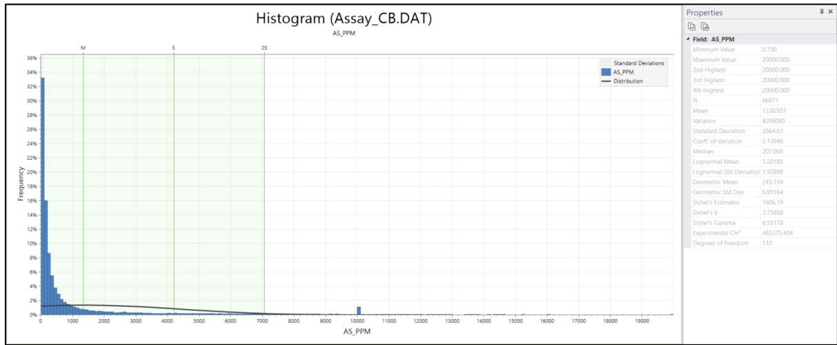
Figure 14.9: Histogram and frequency plot basic statistics (As ppm).
