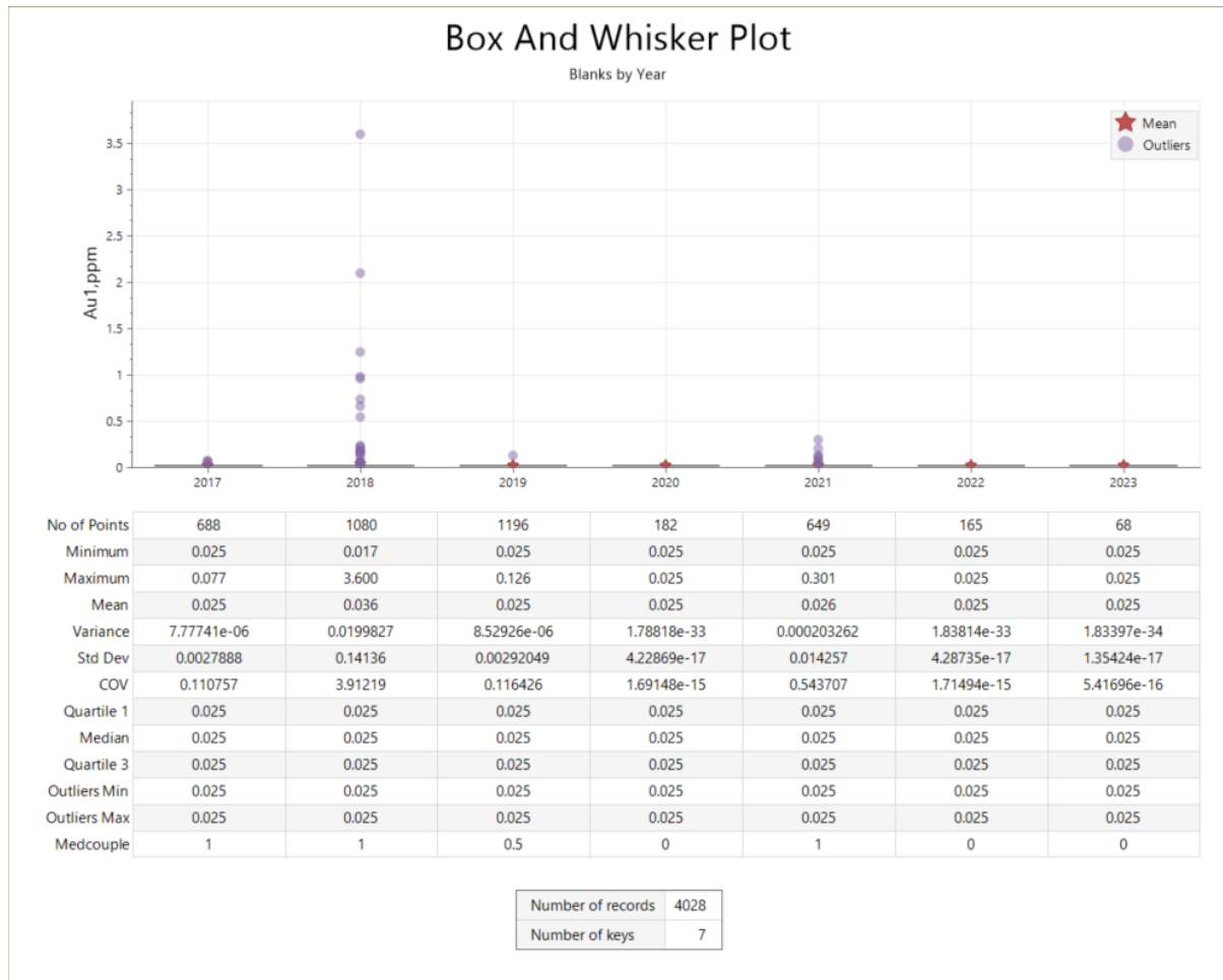
Figure 11.12: QAQC Program, Blanks Results.
