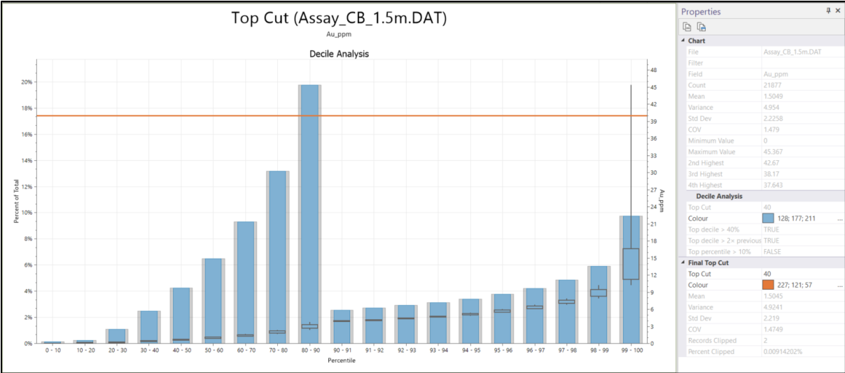
Figure 14.12: Decile analysis showing the top cut statistics for Au.
